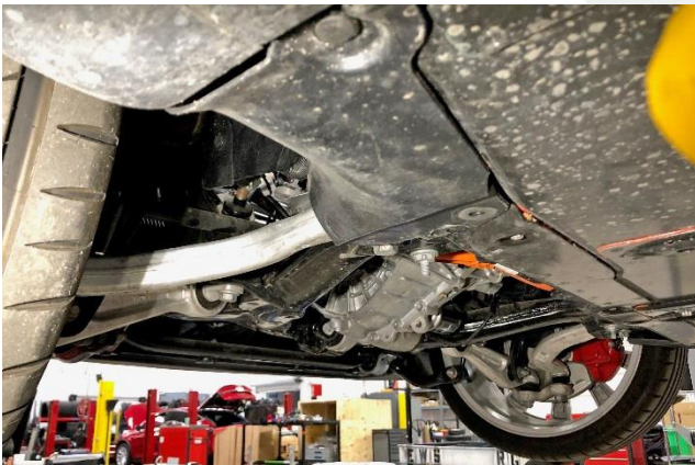
✗ Figure 3 – Front aero shield panel missing
